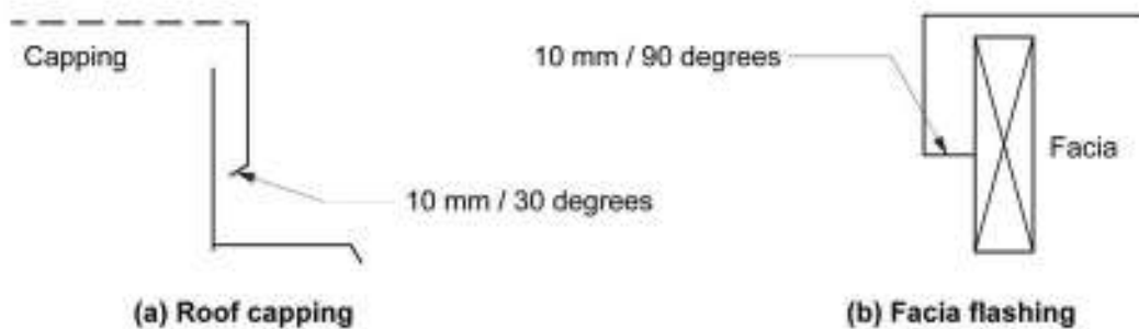
Figure 3.5.1.5 Anti-capillary breaks
