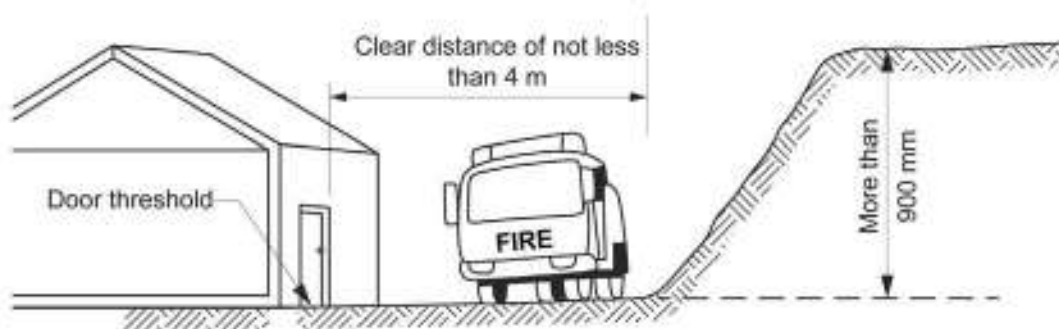
Figure 3.10.4.3d Clear spaces around buildings—Use of a threshold where clear space is not available
