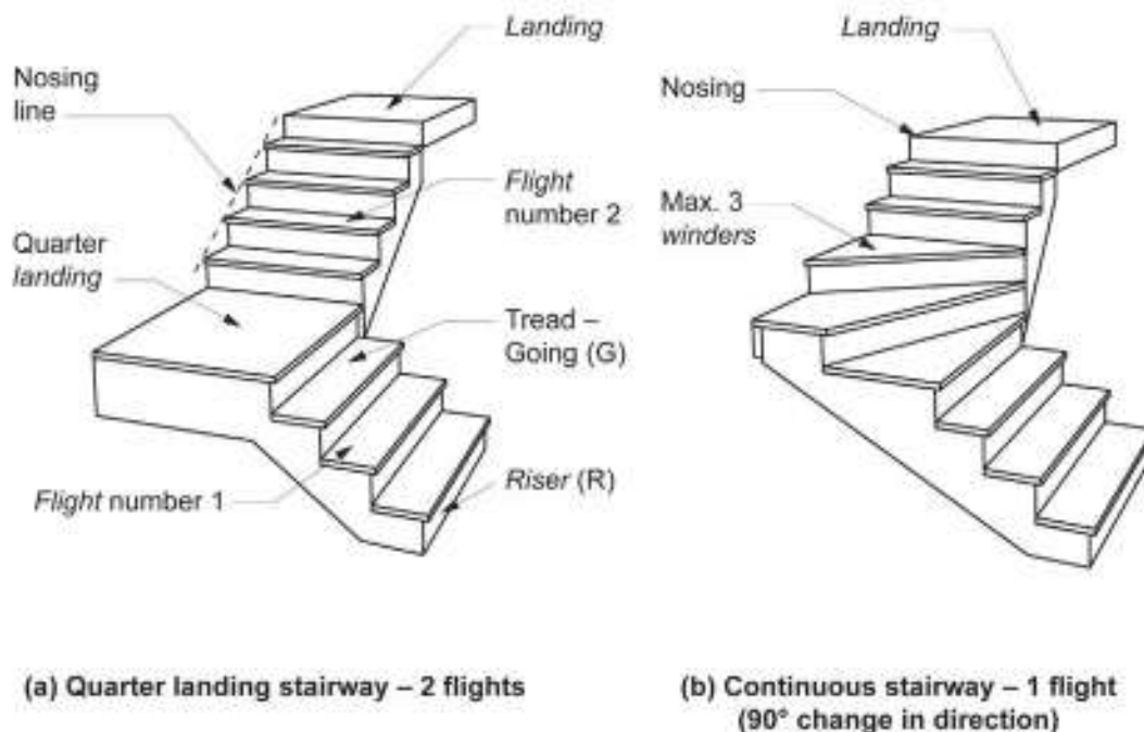
Figure 3.9.1.0 Stairway terms
