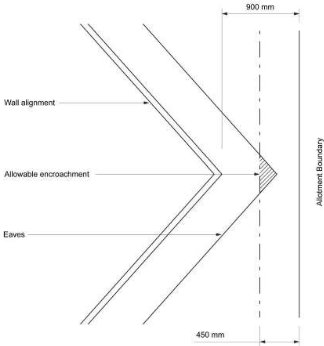
Figure SA 3.7.2.9a Concession for encroachment of eaves
