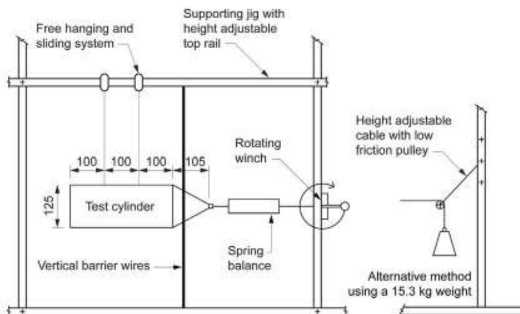
Figure V2.5.1 Apparatus for testing wire barriers
